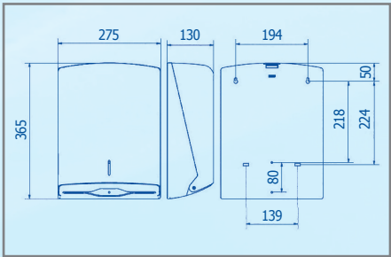
AH33000
